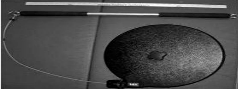
Figure 3.1: PrimusRS 3-dimensional cable motion system
